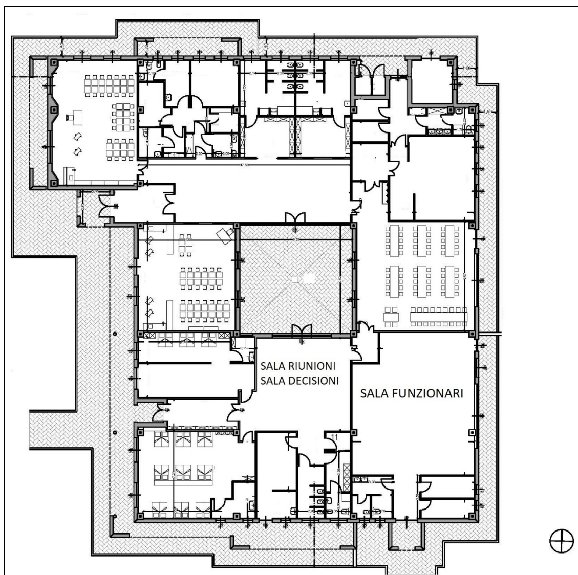
Fig. 21: planimetria C.O.C.
